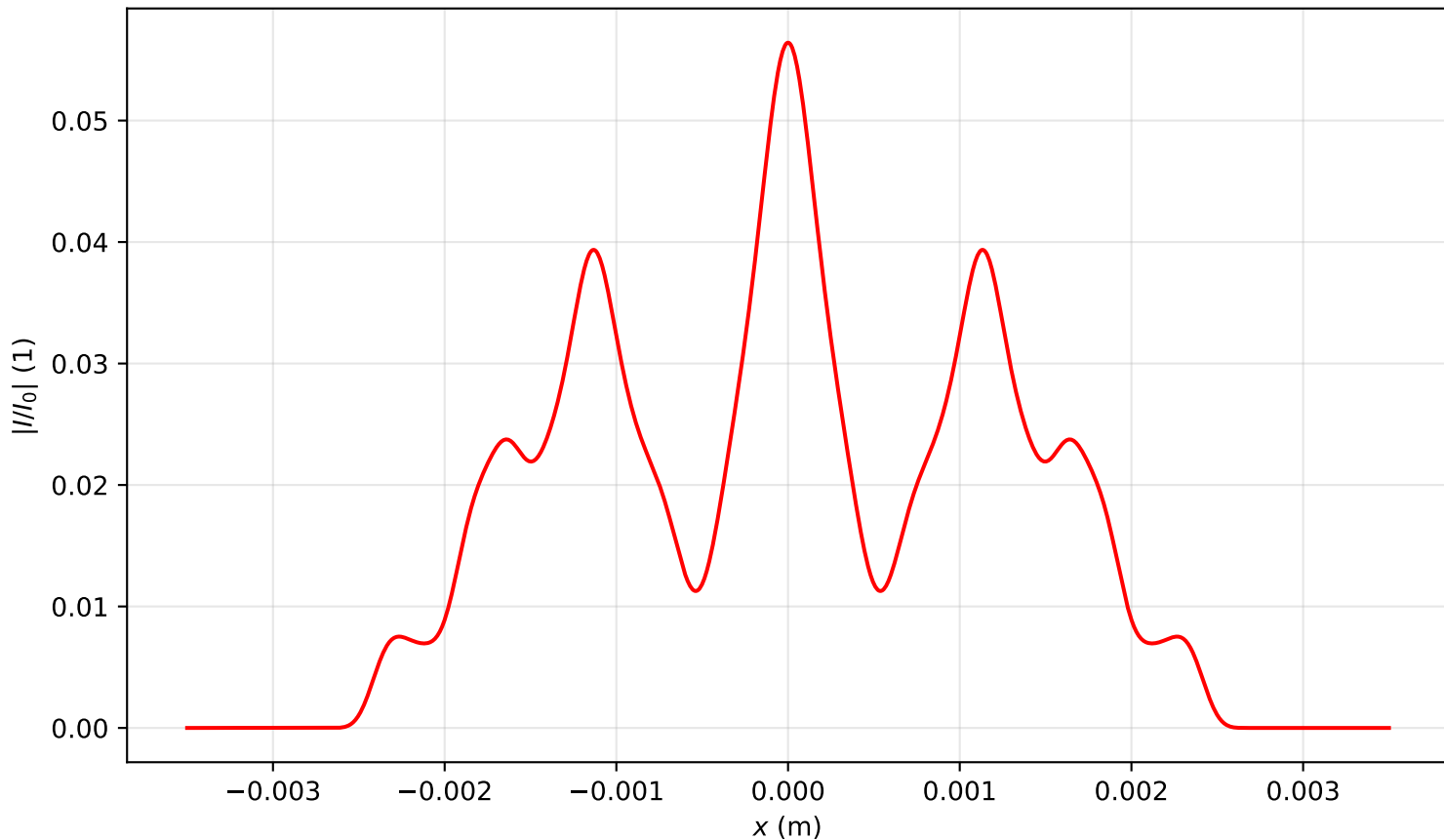
Intensity profile I(x, y = 0, z = 3.821)/I_0 , P_{in}=8.5P_{cr} , artificial time
